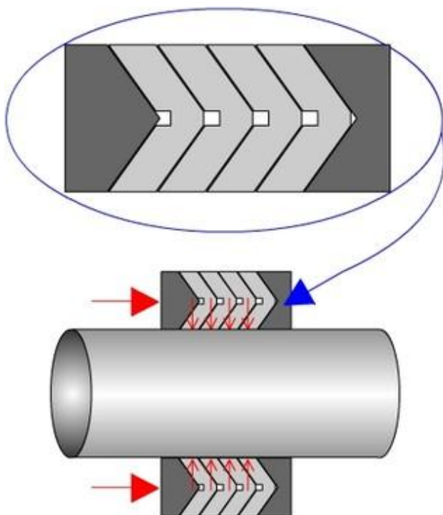
CHEVRON PACKING / 'V' PACKING
